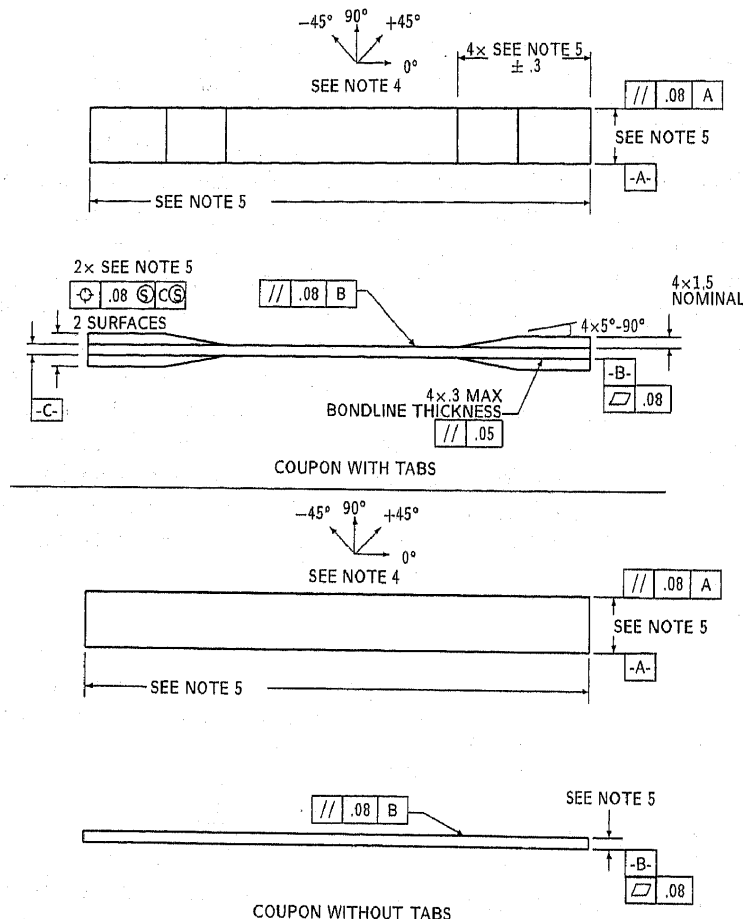
FIG. 2 Tension Test Specimen Drawing (SI)
