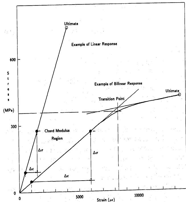
FIG. 5 Typical Tensile Stress-Strain Curves
