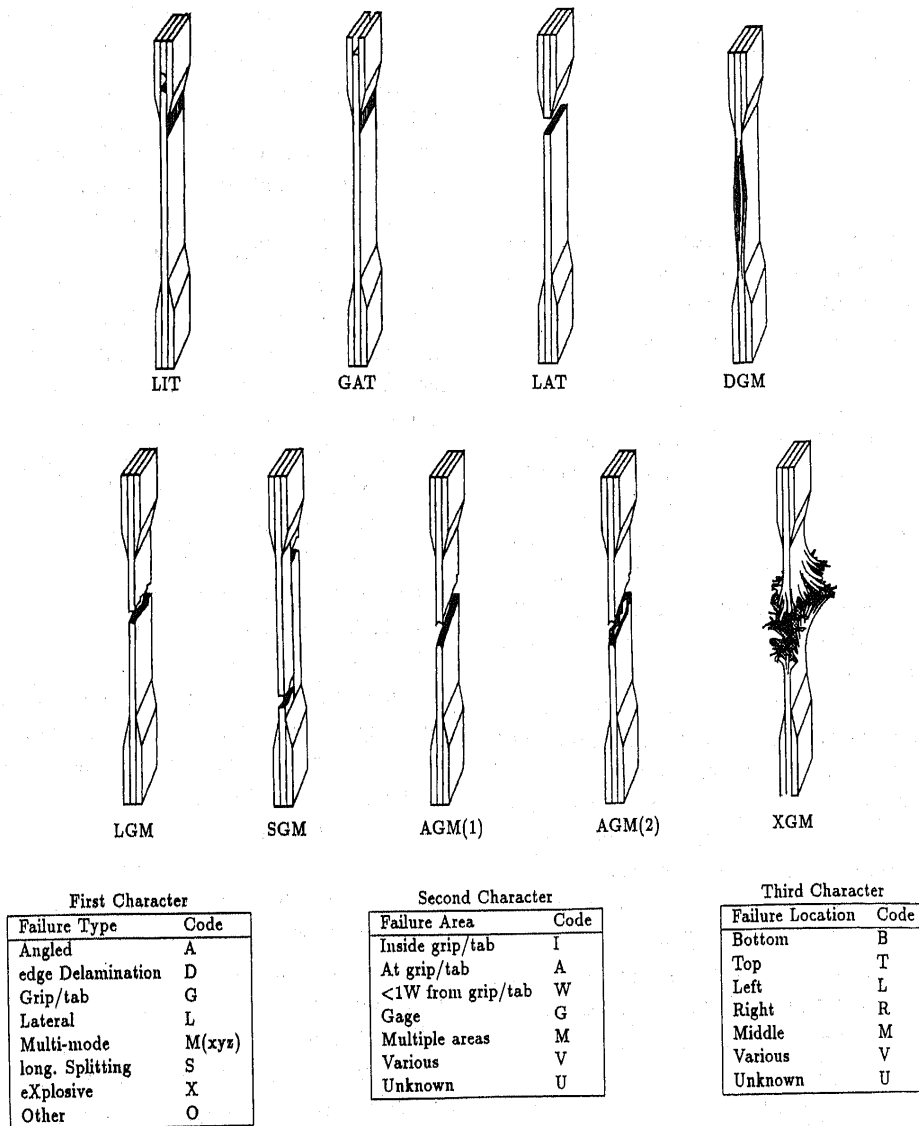
FIG. 4 Tensile Test Failure Codes/Typical Modes
